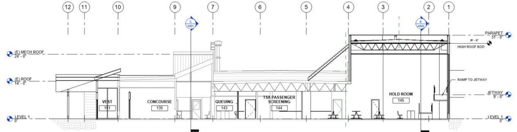
D BUILDING SECTION D A502 1/8" = 1'-0"
