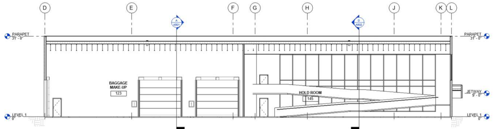
E BUILDING SECTION E A502 1/8" = 1'-0"
